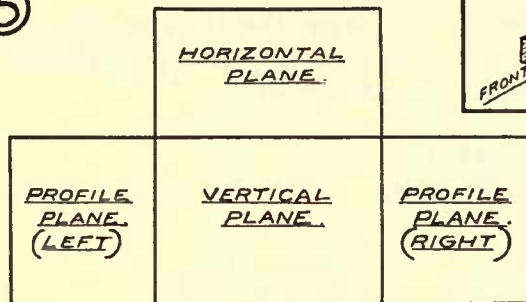
SHOWING PLANES UNFOLDED WHEN LOOKING DIRECTLY AT VERTICAL PLANE.
